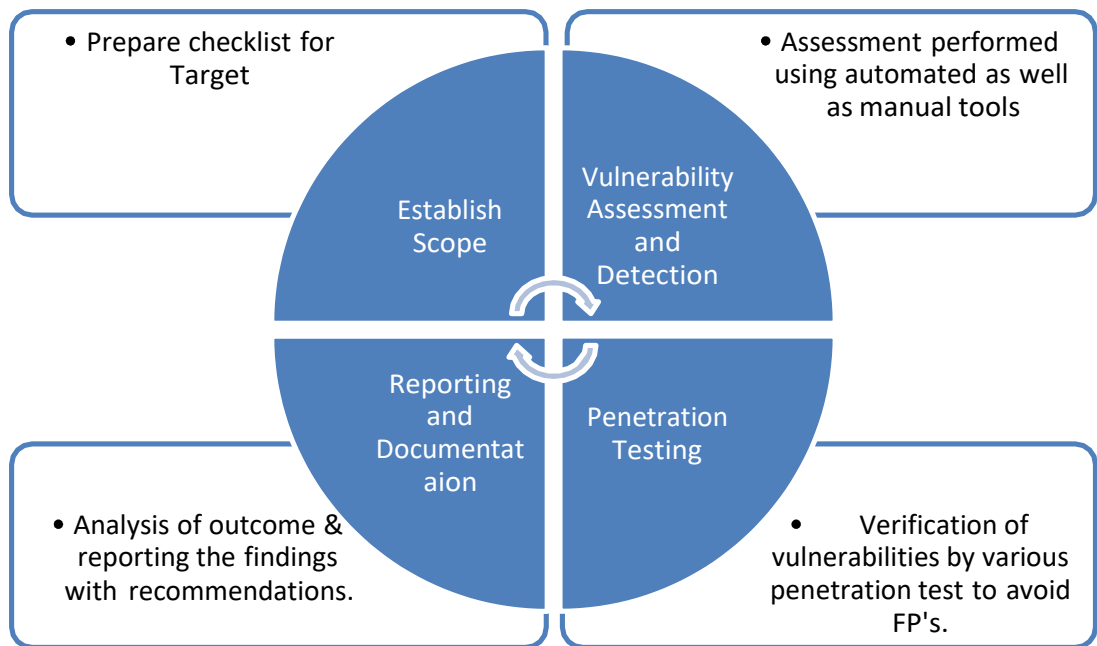
Figure 2.6 VAPT Process
