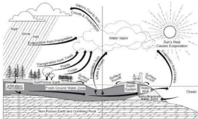
Figure 5 Hydrological cycle
