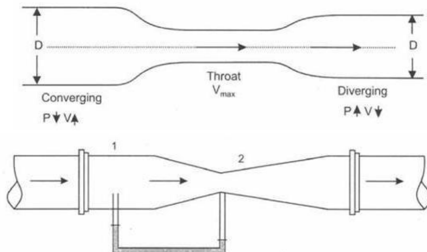
Figure 5 Venturi meter
