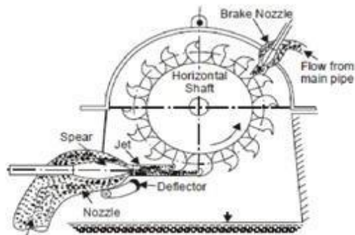
Figure 12 Impulse Turbines
