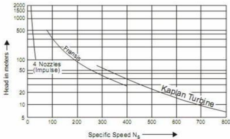
Figure 14 Specific speed versus head
