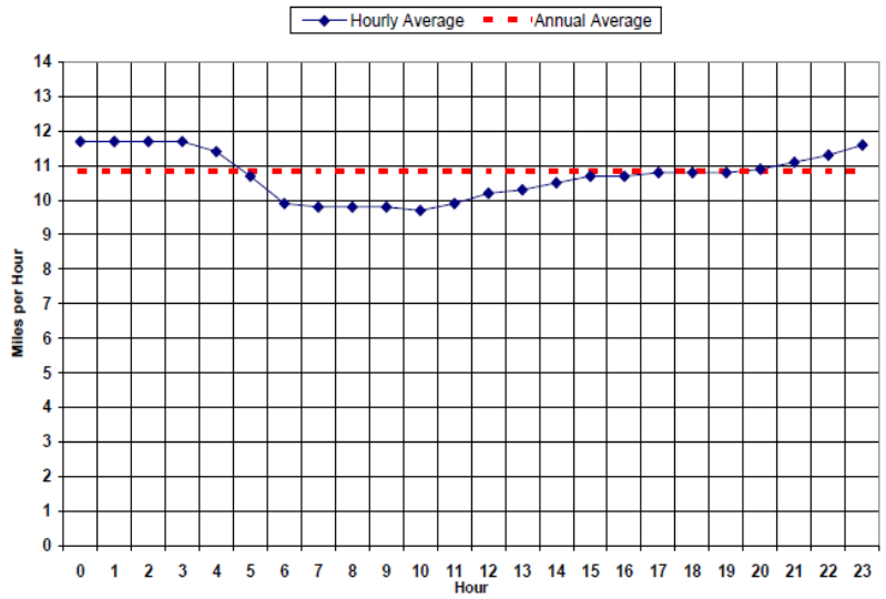
Figure 24: Diurnal wind speed distribution
