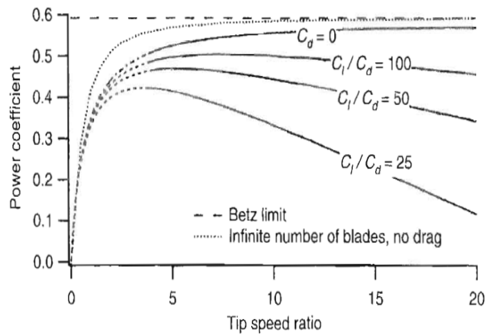
Figure 13: Maximum attainable power coefficient versus C_l/C_d ratio characteristics
