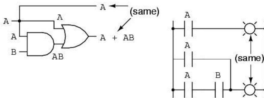
Fig. 5.6 Logical Circuit for Expression A + AB = A
