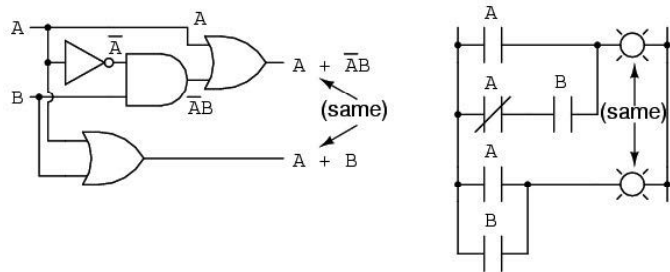
Fig. 5.7 Logical Circuit for Expression
