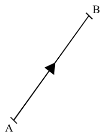
Fig. 4.1 Vector \vec{AB}
