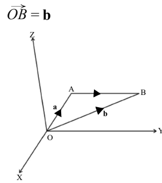
Fig. 4.10 Position Vector
