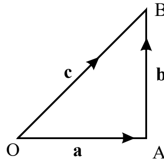
Fig.4.4 Triangle Law
