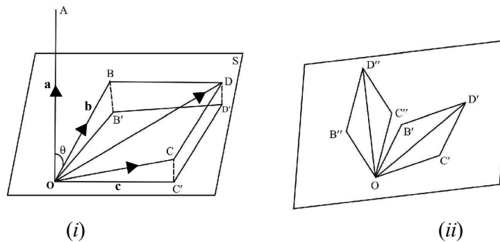
Fig. 4.16 Distributive Law
