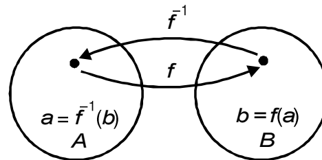
Fig. 3.3 Inverse Function
