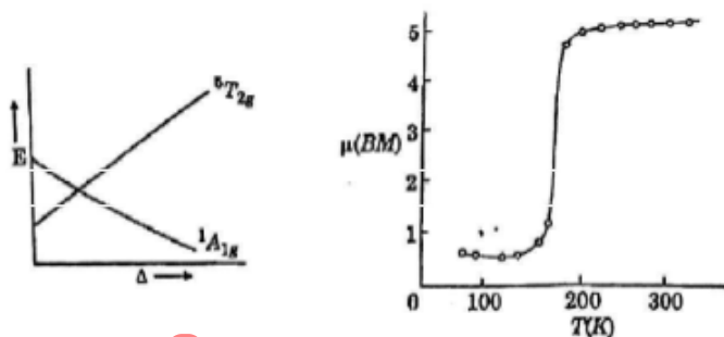
Fig. 2.24 Variation in Magnetic Moment of [Fe(phen)_2(NCS)_2] with Temperature
