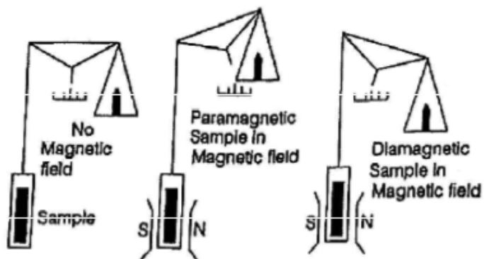
Fig. 2.22 A Paramagnetic Substance Appears to Weigh More in a Magnetic Field while a Diamagnetic Substance Shows Less Weight
