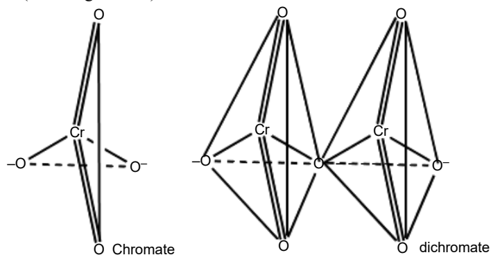
Fig. 5.27 Chromate and Dichromate Ions
