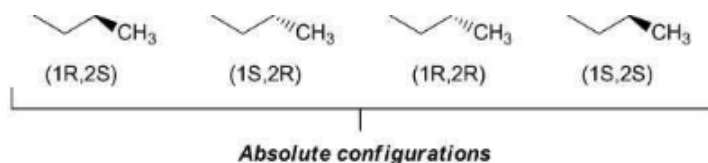
Fig. 2.20 Absolute and Relative Configurations
