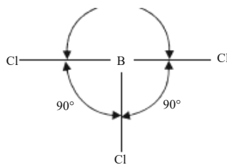
(a) T-shaped geometry of \text{BCl}_3 molecule (bp-bp) repulsions at 90^\circ = 2 , bp-bp repulsions at 180^\circ = 1
