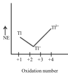
Fig. 3.19 Construction of Frost Diagram for Thallium from Latimer Diagram
