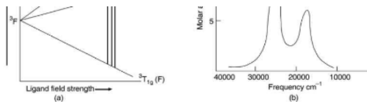
Fig.2.12 (a) Transitions for V^{3+} ( d^2 ) Ion and (b) Absorption Spectrum of a d^2 Complex [V(H_2O)_6]^{3+}
