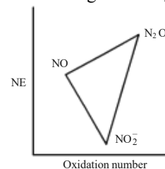
Fig. 3.17 Frost Diagram Showing Comproportionation
