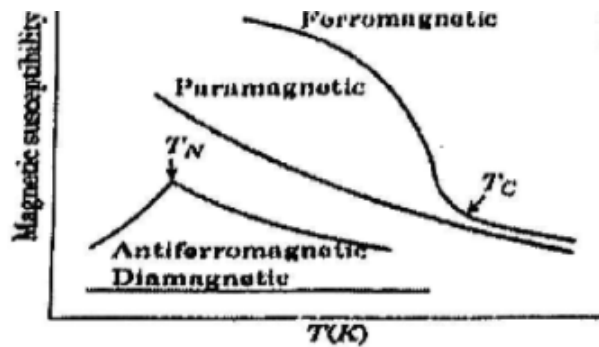
Fig. 2.27 Variation of Magnetic Susceptibility with Temperature for Diamagnetic, Paramagnetic, Ferromagnetic and Antiferromagnetic Substances
