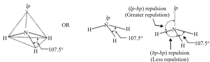
Fig. 1.10 (a) Trigonal Pyramidal Shape of \text{NH}_3 Molecule, lp Indicates a Lone Pair of Electrons. (b) To Explain why H-N-H Bond Angle is \text{NH}_3 is Less than the Tetrahedral Bond Angle (= 109.5^\circ ). lp Indicates a Lone Pair of Electrons on N-Atom
