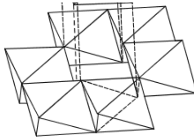
Fig. 5.35 Structure of [Mo_6O_{24}]^{12-} with Large Central Cavity
