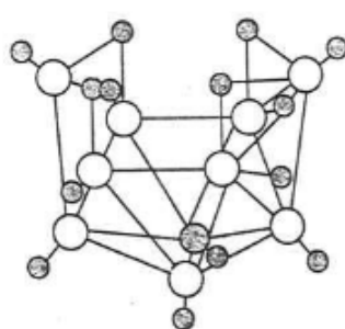
Decaborane-14, B_{10}H_{14}
