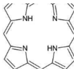
Porphine
