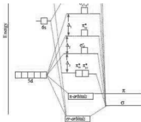
Fig. 1.26 The MO Diagram for [PtCl_4]^{2-} Ion
