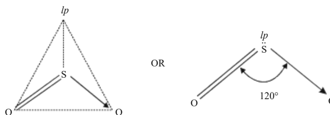
Fig. 1.9 Angular Shape of SO_2 Molecule
