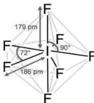
Structure of IF_7 - Pentagonal Bipyramidal
