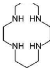
Cyclam
