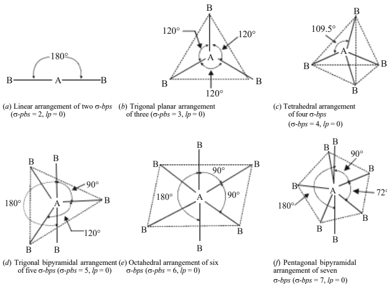
Fig. 1.1 Spatial Arrangement of 2, 3, 4, 5, 6 and 7 \sigma -bonding Electron Pairs ( \sigma\text{-bps} ) Round the Central Atom (A). The Central Atom is not Surrounded by Any Lone Pair of Electrons (lps). B are the Atoms with which Central Atom (A) is Linked by \sigma\text{-bps} .
