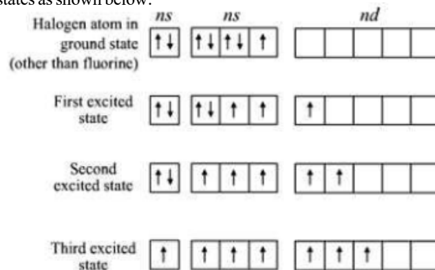
Fig. 5.23 Excited States of Halogen Atoms
