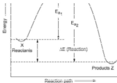
Fig. 3.1 Energy Profile Diagram
