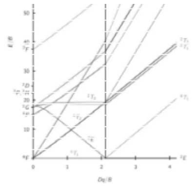
d 7 Electron Configuration
