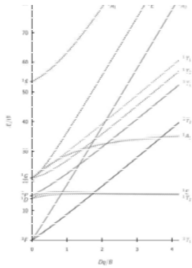
d 2 Electron Configuration
