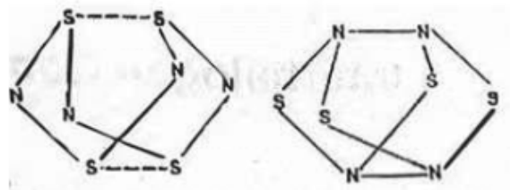
Fig. 5.22 Crown-Shaped Ring of Sulphur Nitride
