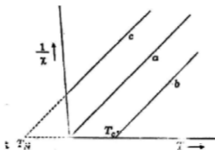
Fig. 2.25 Graph Plotted Between Reciprocal of Magnetic Susceptibility and Temperature in Kelvin
