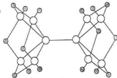
Decaborane-16, B_{10}H_{16}
