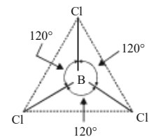
(b) Trigonal planar geometry of \text{BCl}_3 molecule (bp-bp repulsions at 120^\circ = 3 )
