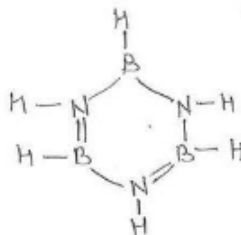
Fig. 5.12 Borazine
