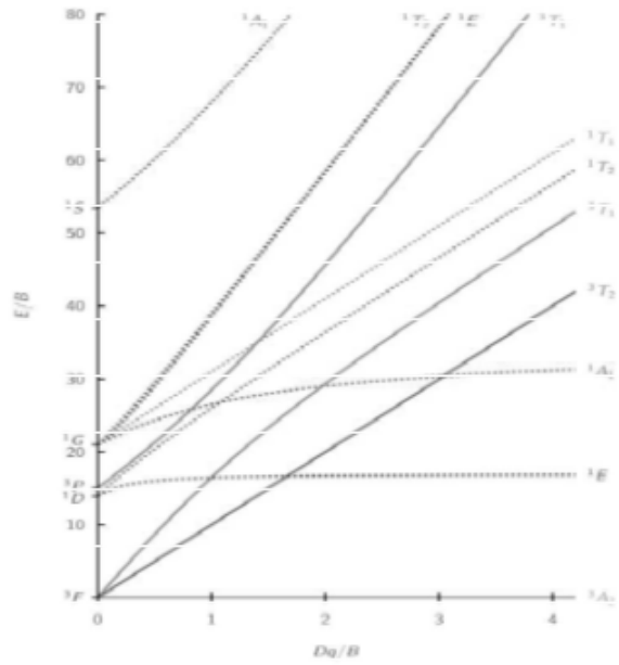
d 8 Electron Configuration
