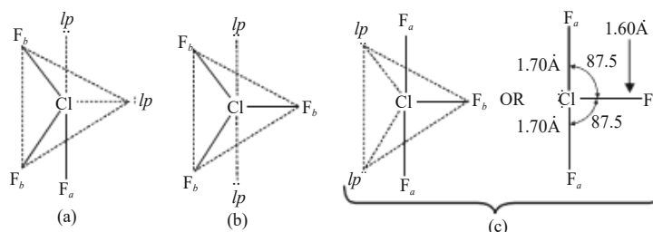
Fig 1.14 Three Possible Geometries of ClF_3 Molecule
