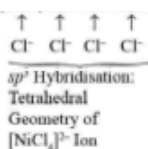
Fig. 3.12 sp^3 Hybridisation of \text{Ni}^{2+} Ion in [\text{NiCl}_4]^{2-} Ion which has Tetrahedral Geometry
