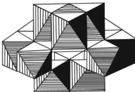
Fig. 5.31 Structure of [\text{W}_{12}\text{O}_{42}]^{12-} Unit in Paratungstate Ion
