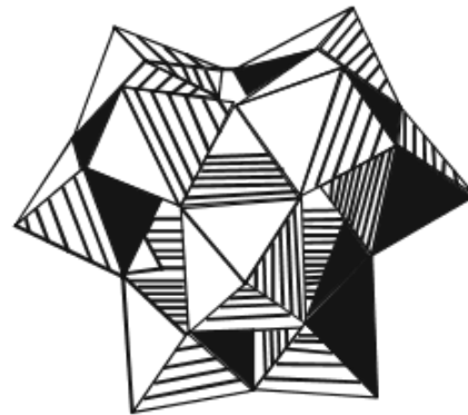
Fig. 5.34 The Structure of Series A 12-molybdo and 12-tungsto Heteropolyanions of General Formula [X^{n+}Mo_{12}O_{40}]^{(8-n)-}
