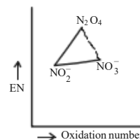
Fig. 3.16 Frost Diagram Showing Disproportionation of \text{N}_2\text{O}_4
