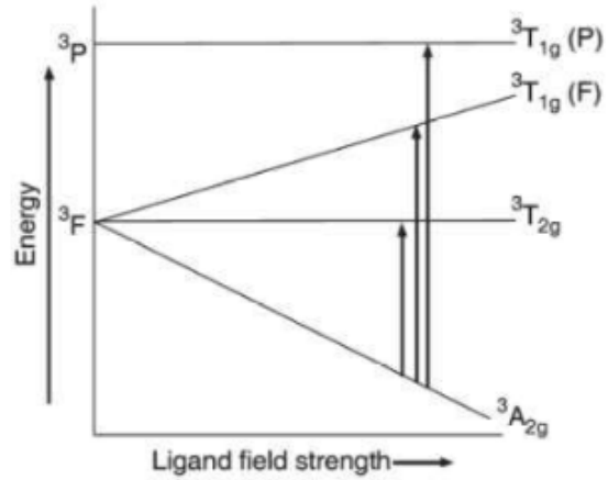
Fig. 2.13 Energy Level Diagram of d^8 Ion
