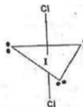
Fig. 5.24 Structure of ICl_2^-
