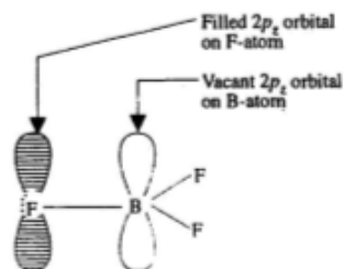
Fig. 3.13 Structure of BF_3 Molecule
