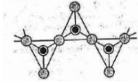
Fig. 5.19 (\text{SiO}_3)_n^{-2n}
