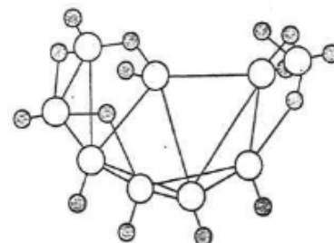
Nonaborane-15, B_9H_{15}
