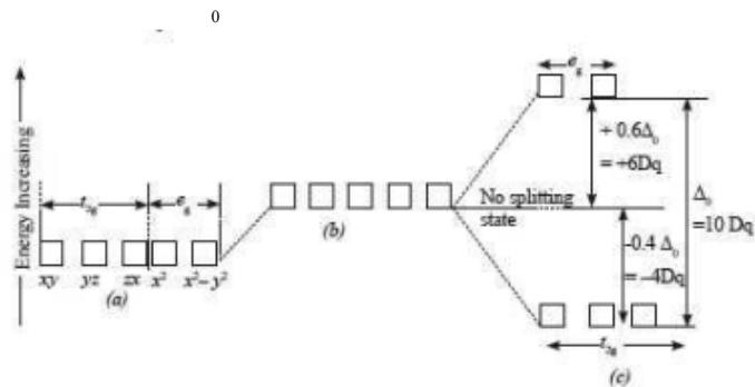
Fig. 1.22 Splitting of Five d -orbitals in an octahedral Complex. (a) Five Degenerate d -orbitals on the Central Metal Cation which are free from any Ligand Field. (b) Hypothetical Degenerate d -orbitals at a Higher Energy Level (c) Splitting of d -orbitals into t_{2g} and e_g orbitals Under the Influence of Six Ligands in Octahedral Complex.
