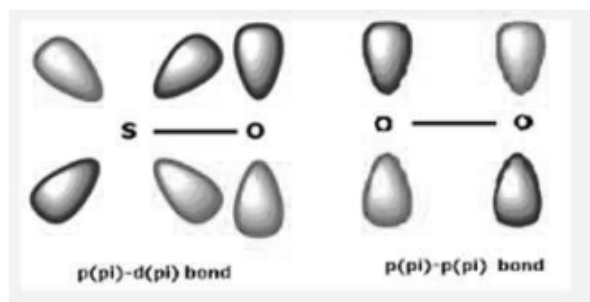
Fig. 1.20 p(\pi) - p(\pi) or p(\pi) - d(\pi) Bonds
