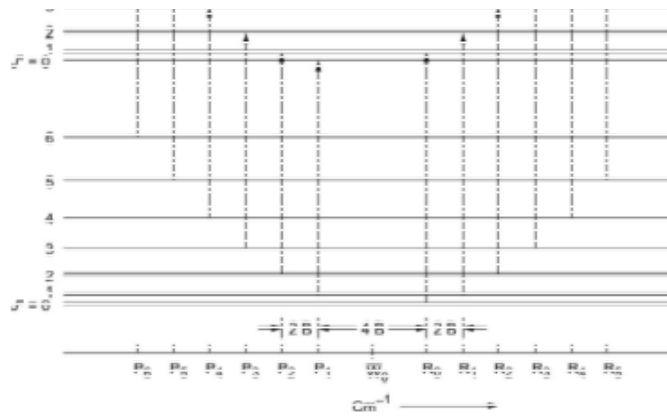
Fig. 2.7 Vibration-Rotation Spectrum of HBr for Transition From v = 0 to v = 1
