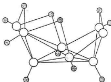
Octaborane-12, B_8H_{12}
