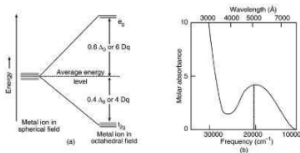
Fig. 2.15 Splitting of Energy Levels for d^1 Configuration in an Octahedral Field and (b) Visible Spectrum of [\text{Ti}(\text{H}_2\text{O})_6]^{3+} Complex Ion
