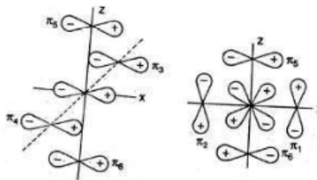
Fig. 1.29. The Formation of Metal-Carbon \pi -Bond
