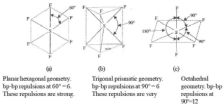
Fig. 1.7 Three Possible Geometries of SF_6 Molecule
