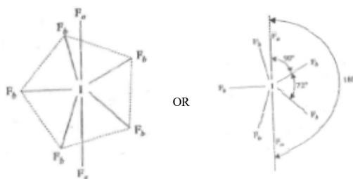
Fig. 1.8 Pentagonal Bipyramidal Structure of IF_7 Molecule
