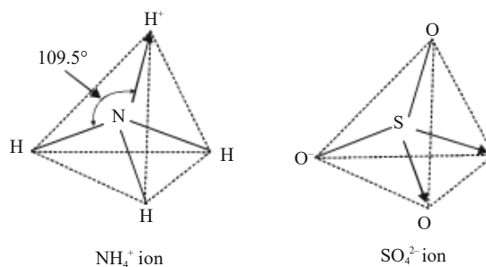
Fig. 1.5 Tetrahedral Shape of \text{NH}_4^+ and \text{SO}_4^{2-} Ions.
