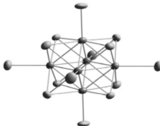
Fig. 5.26 Structure of \text{Mo}_6\text{Cl}_{14}^{2d}
