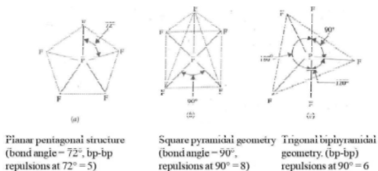
Fig. 1.6 Three Possible Geometries of PF_5 Molecule
