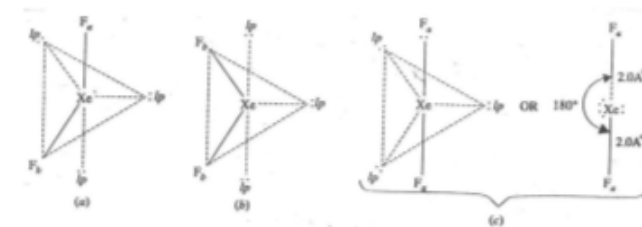
Fig 1.15 Three Possible Geometries of \text{XeF}_2 Molecule
