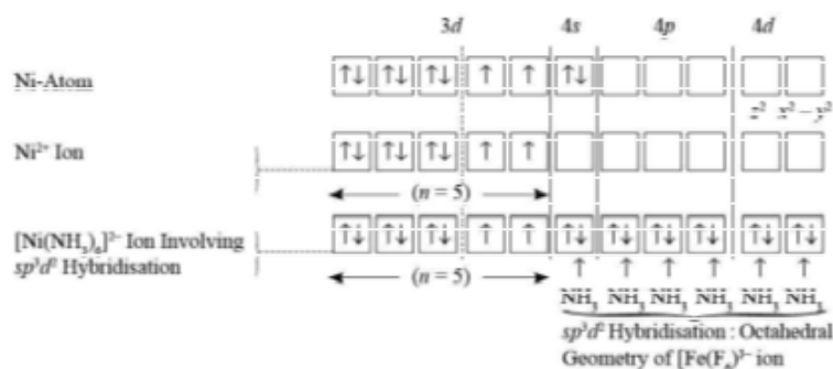
Fig. 3.5 Formation of [\text{Ni}(\text{NH}_3)_6]^{2+} Ion by sp^3d^2 Hybridisation (Outer-Orbital Octahedral Complex Ion).
