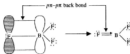
Fig. 3.14 Formation of p\pi - p\pi Back Bond in BF_3 Molecule
