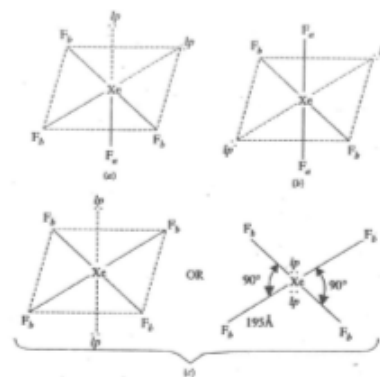
Fig. 1.17 Three Different Geometries of XeF_4 Molecule
