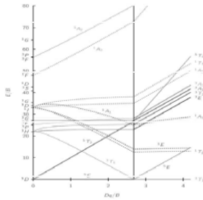
d 4 Electron Configuration
