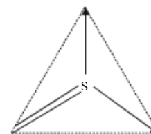
Trigonal planar geometry of \text{SO}_3 molecule
