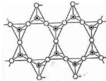
Fig. 5.20 Chain (\text{Si}_4\text{O}_{11})_n^{-2n}
