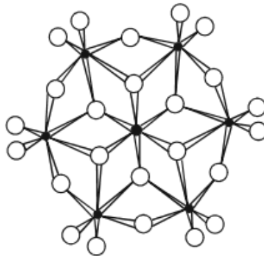
Fig. 5.36 Structure of [CrMo_6O_{24}H_6]^{3-} Ion
