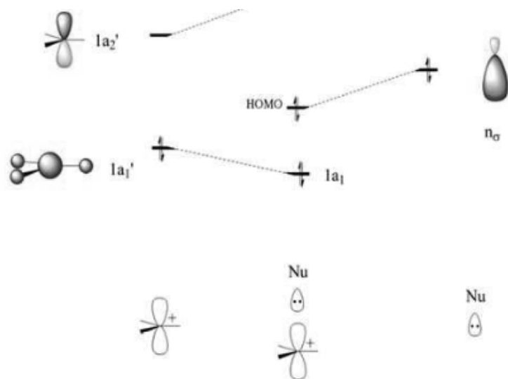
Fig. 1.19 Orbital Interaction Diagram for Nucleophilic Addition to \text{CH}_3^+
