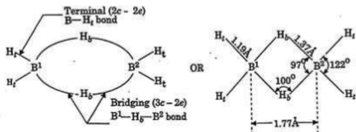
Fig. 5.2 Hydrogen-Bridged Structure of Diborane Molecule, B_2H_6
