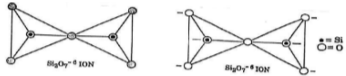
Fig. 5.17 Pyrosilicate Anion
