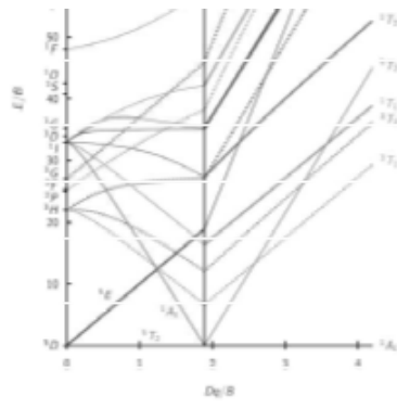
d 6 Electron Configuration
