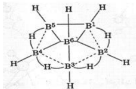
Fig. 5.10 Structure of Hexaborane-10, B_6H_{10}
