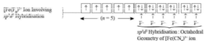
Fig. 3.4 Formation of [\text{FeF}_6]^{3-} Ion by sp^3d^2 Hybridisation (Outer-Orbital Octahedral Complex Ion).
