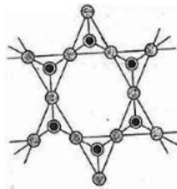
Fig. 5.21 (\text{Si}_2\text{O}_5)_n^{-2n}
