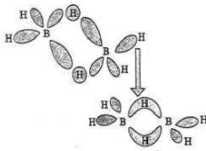
Fig. 5.5 Formation of Three-Centre Bonds in Diborane
