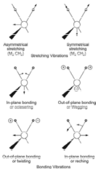
Fig. 2.5: Vibrational Modes for a \text{CH}_2 Group (+ and - Indicate Movement Perpendicular to the Plane of the Page)
