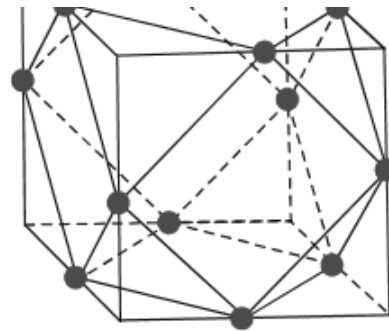
Fig. 5.33 Arrangement of W Ions in [SiW_{12}O_{40}]^{4-} Ion
