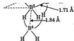
Fig. 5.6 Structure of Tetraborane, B_4H_{10}
