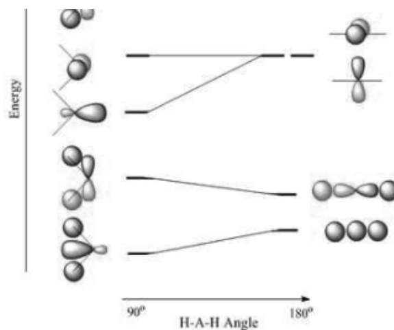
Fig. 1.18 A Walsh Diagram for an AH_2 Molecule
