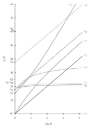
d 3 Electron Configuration
