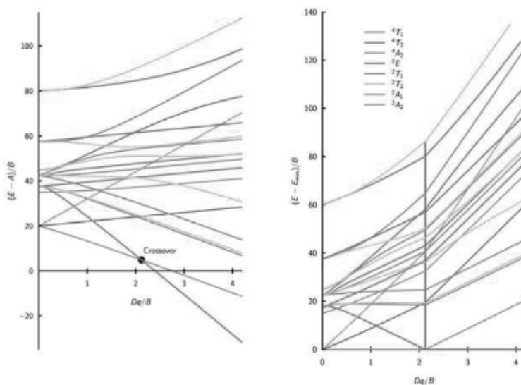
Fig. 2.18 Tanabe–Sugano Diagram
