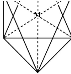
Fig. 5.28 MoO_6/WO_6 Octahedron
