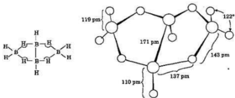
Fig. 5.7 Structure of Tetraborane, B_4H_{10}
