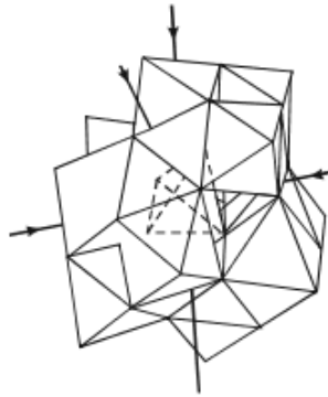
Fig. 5.32 Structure of 12-Molybdoheteropolyanionic Species
