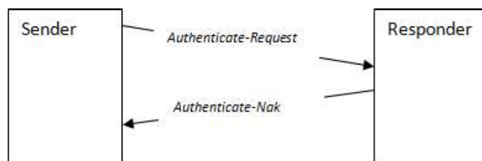
Figure 16: Authenticate-Nak when authentication is not successful
